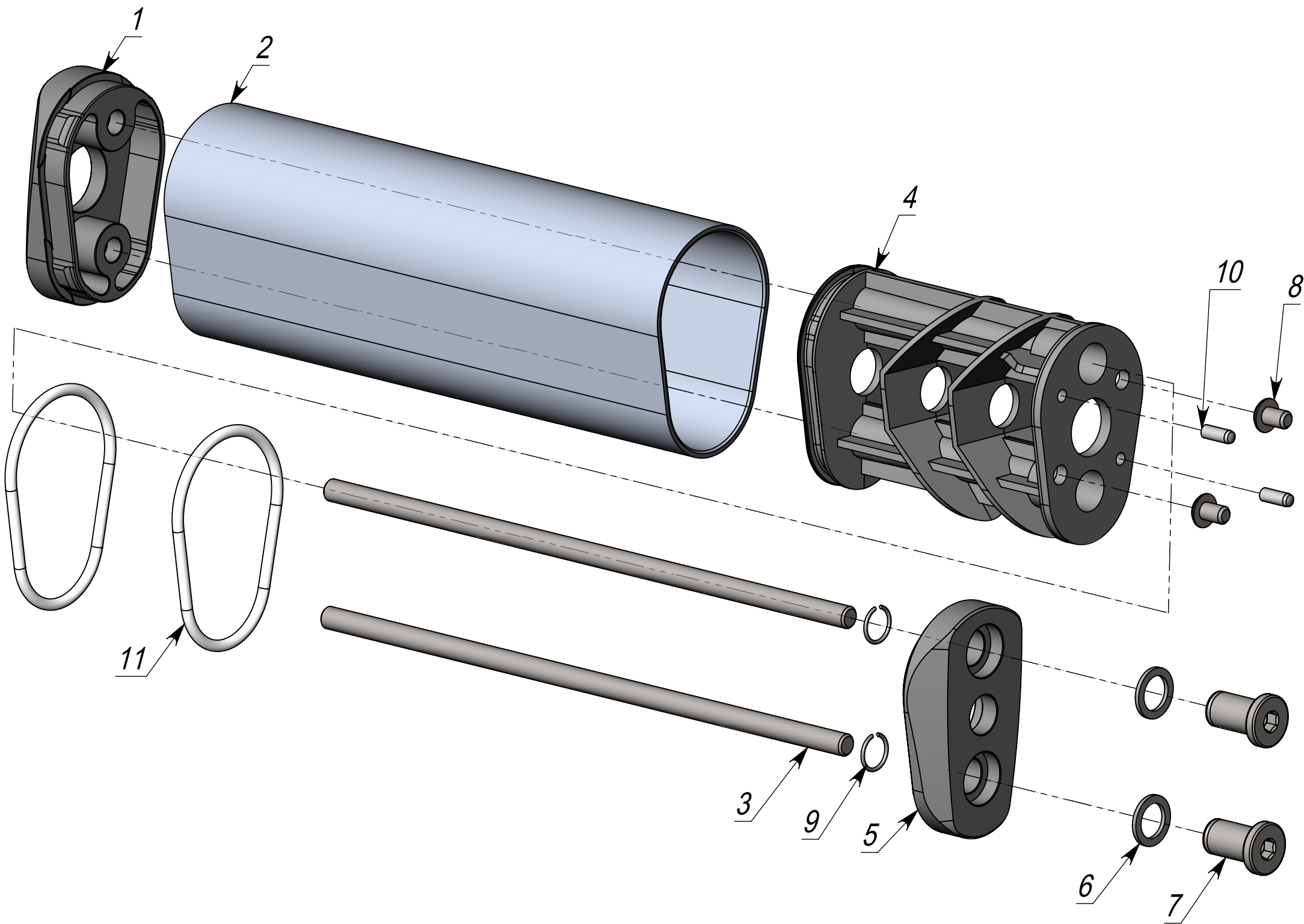
LSA237000 Suppressor
